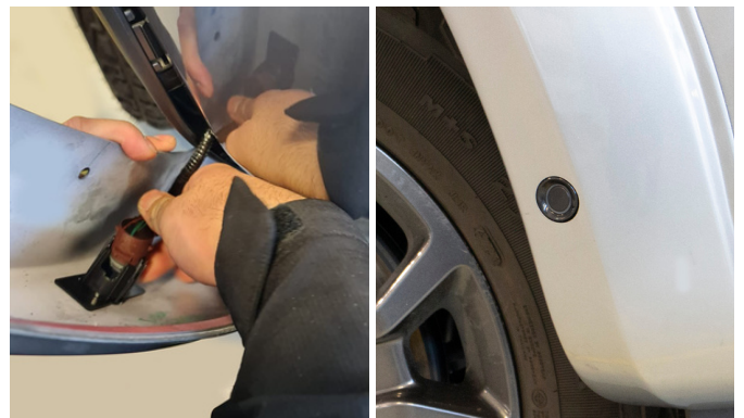
OEM Sensor Mount
